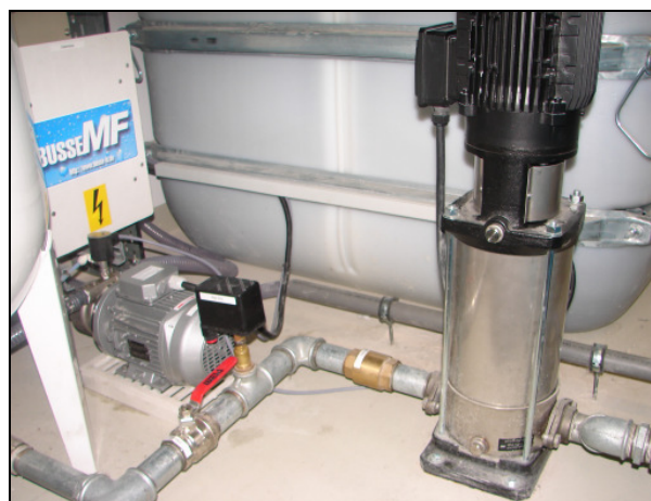
Service water post-treatment with booster pump
