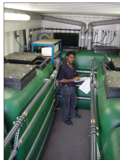
Installation of the system in a 20' container
