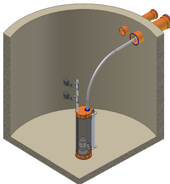
Septic tank with pump
