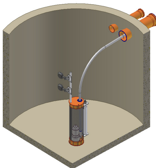
Septic tank with pump
